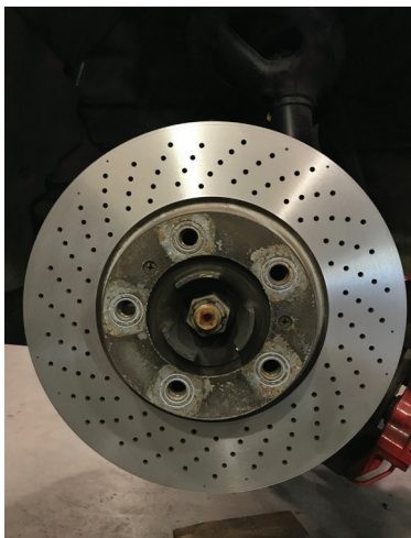
AFTER Match-Machining
